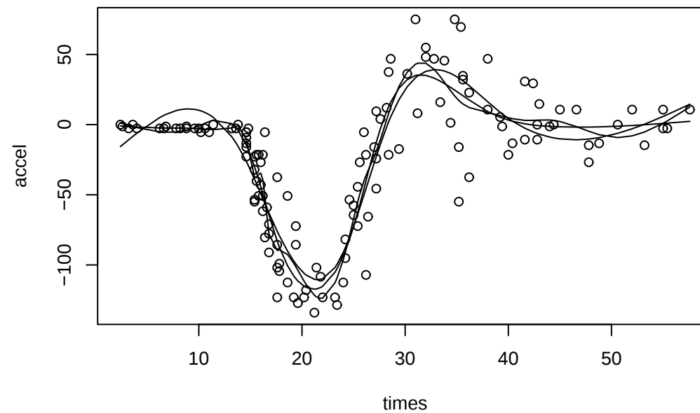
Cubic Splines
