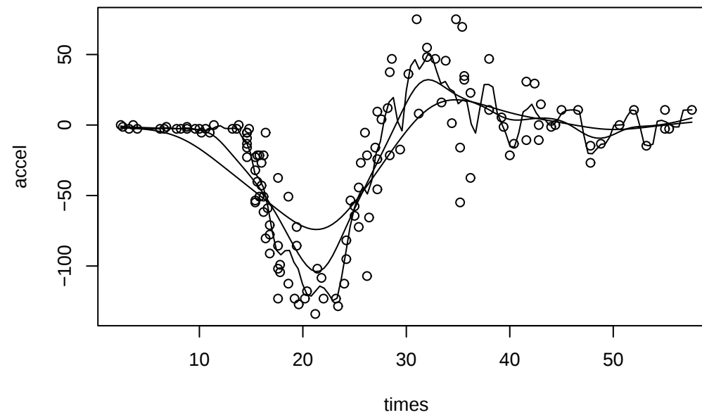
Kernel Smoothing
