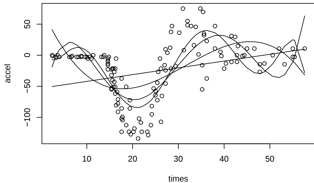
Polynomials
