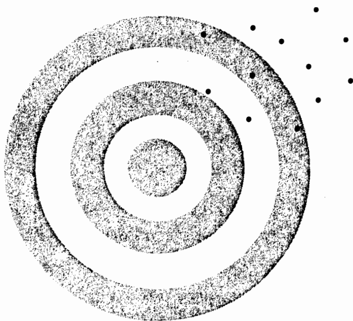
(c) High bias, low precision
