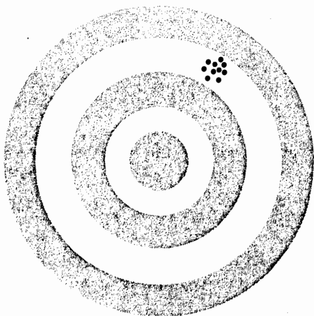
(a) High bias, high precision
