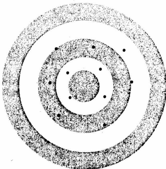
(b) Low bias, low precision
