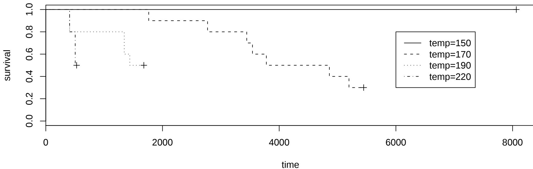
Kaplan–Meier estimators (Motor data)
