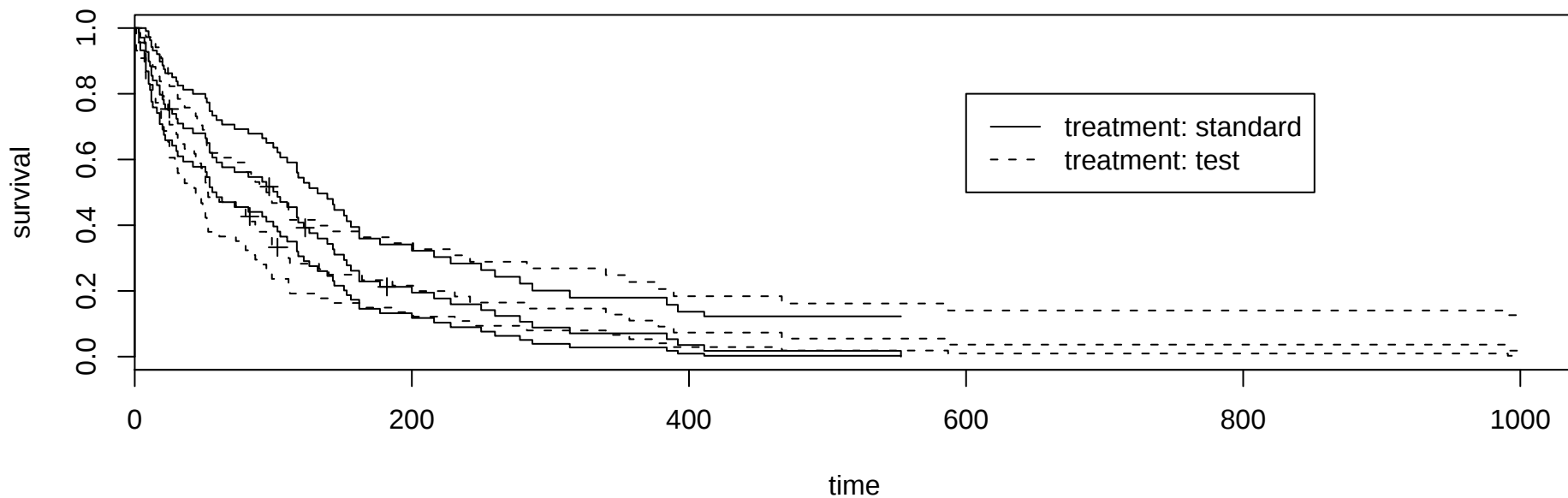
Kaplan-Meier estimators (VA data, with 95% confidence band)
