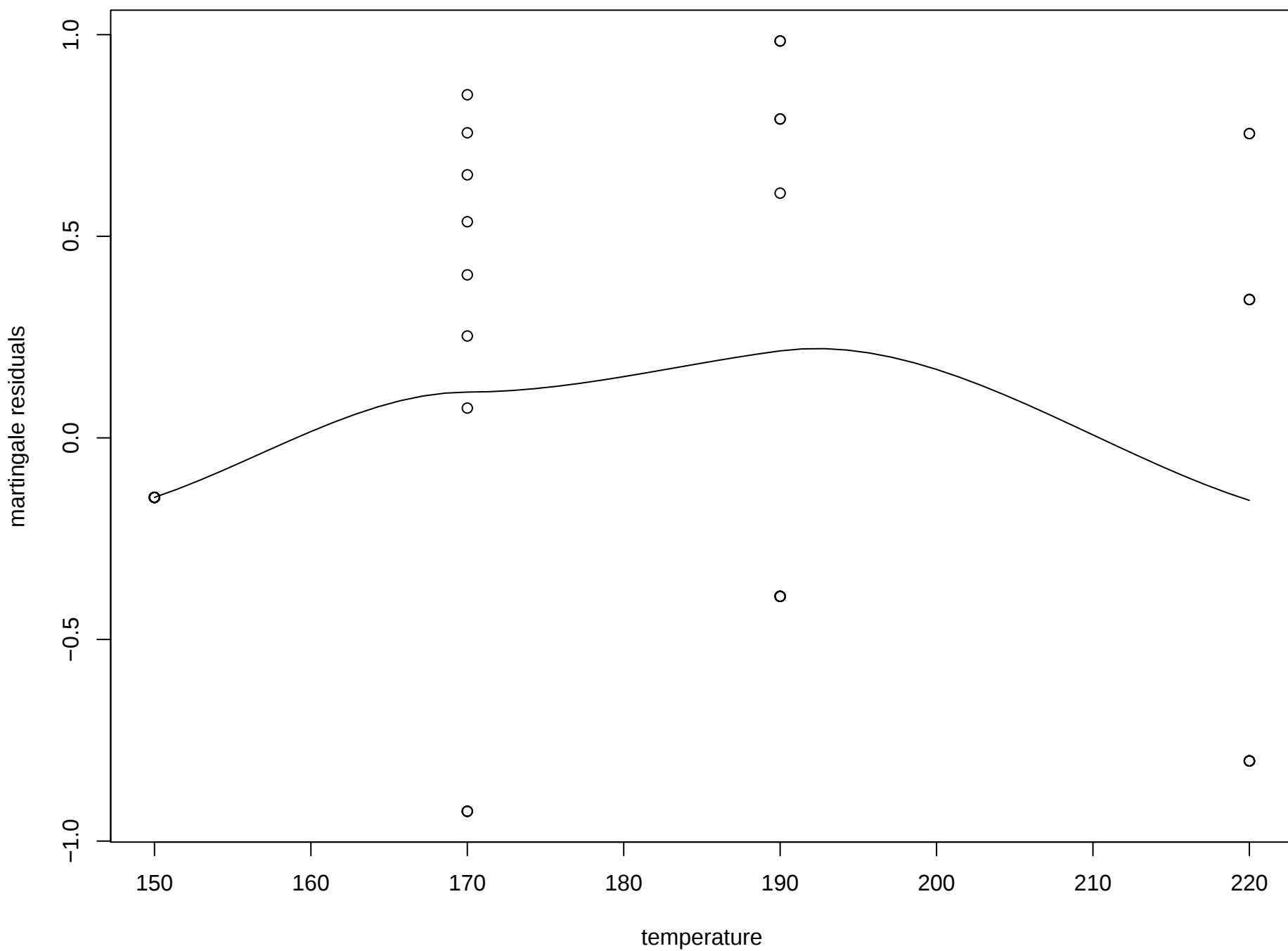
Residual Plot
