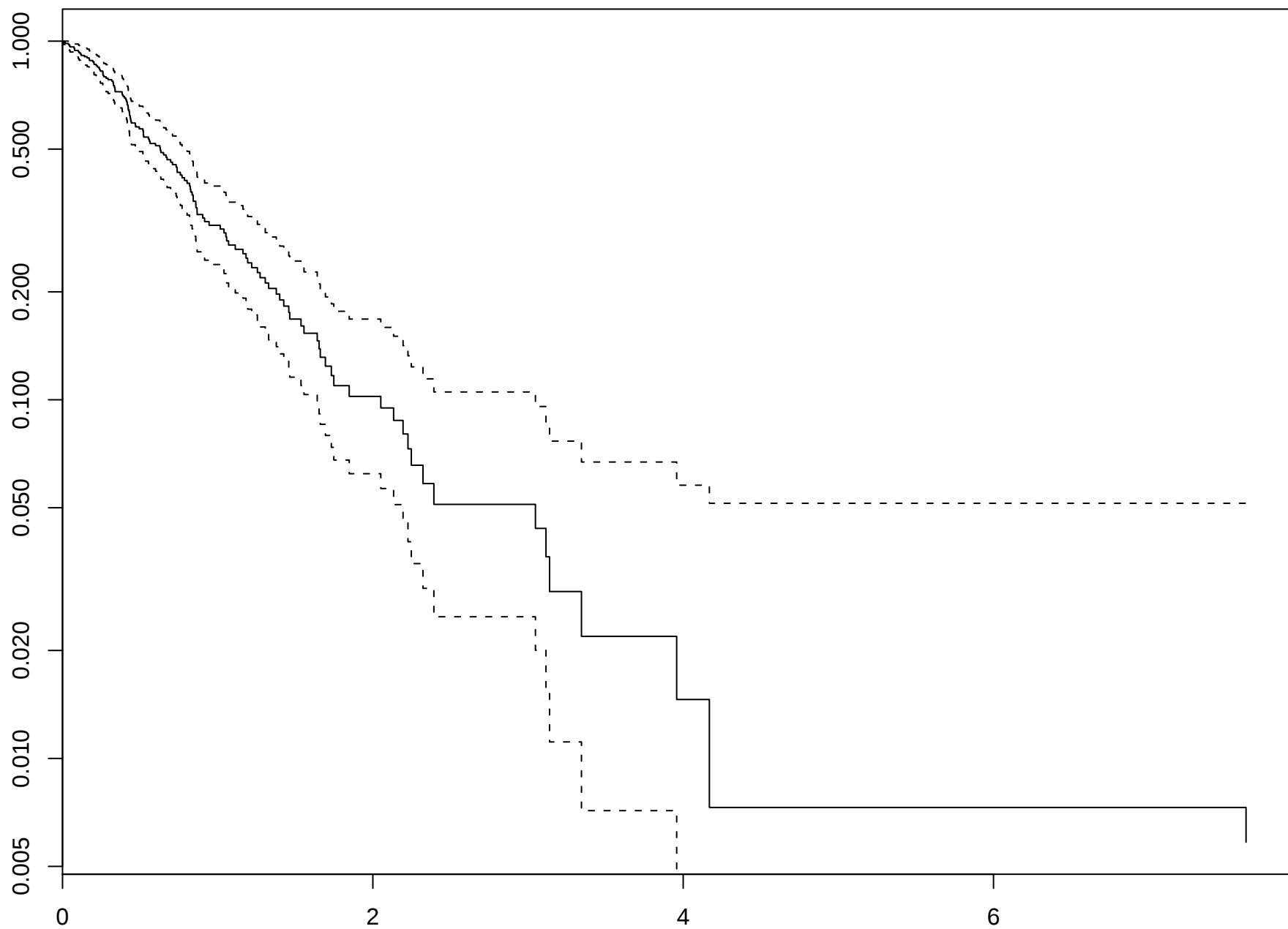
A log plot of S(t)
